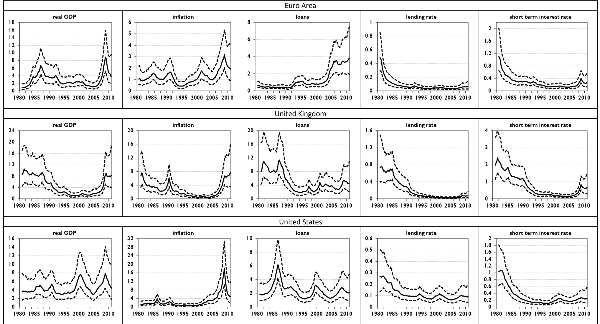
Chart 2 - Stochastic volatility
