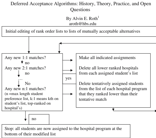
Fig. 1 The 1952 deferred acceptance algorithm (from Roth 1984)
